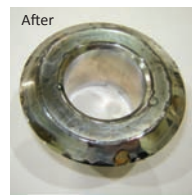
Chrome and plastic parts after 100 hours of testing.
